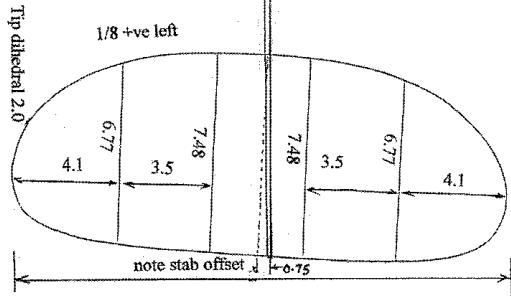
Template for stab 18" flat
